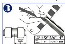
3. Mark the insertion depth
